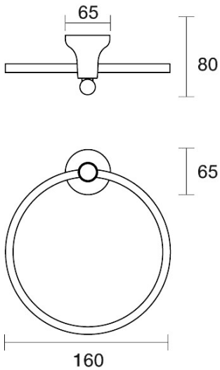
Bell Towel Ring Holder E32.031.1.14 - Gold / Ivory
