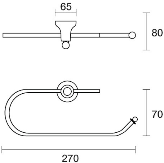
Bell Guest Towel Holder E32.041.1.04 - Chrome / Ivory
