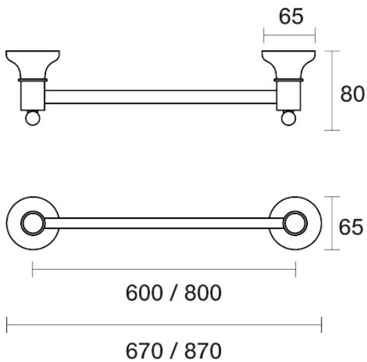
Bell Towel Rail Single 870mm E32.071.2.03 - Chrome / White
