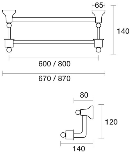
Bell Towel Rail Double 870mm E32.072.2.01 - Chrome
