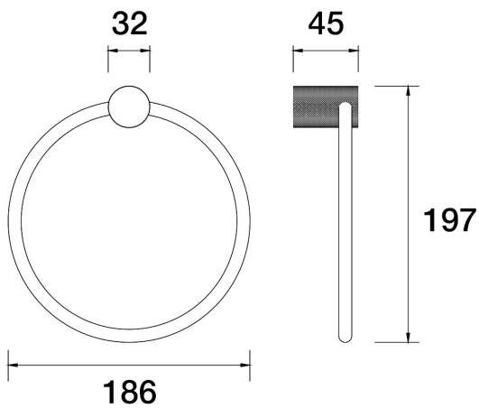
IDK Towel Ring Holder E38.031.1.26 - Black Sapphire
