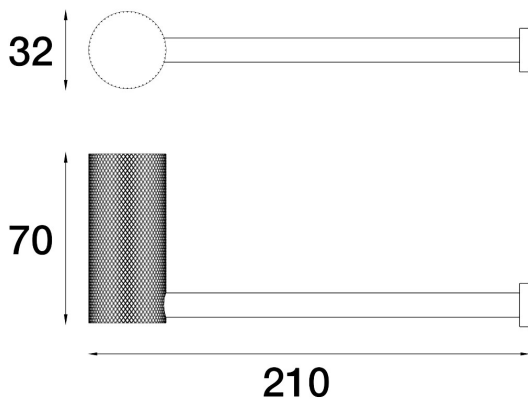
IDK Guest Towel Holder E38.041.1.21 - Brushed Rose Gold
