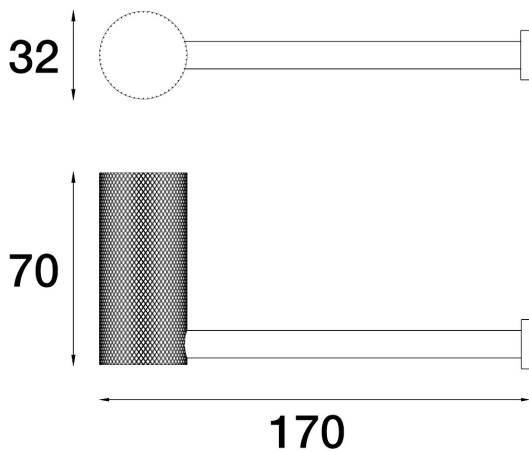
IDK Toilet Roll Holder E38.051.1.52 - Burnished
