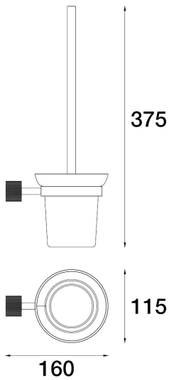
IDK Toilet Brush Holder E38.052.1.39 - Antique Bronze
