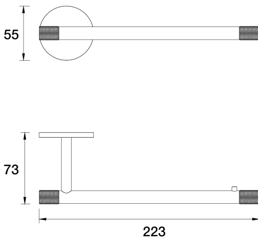
Elm Guest Towel Holder E40.041.1.25 - Brushed Nickel
