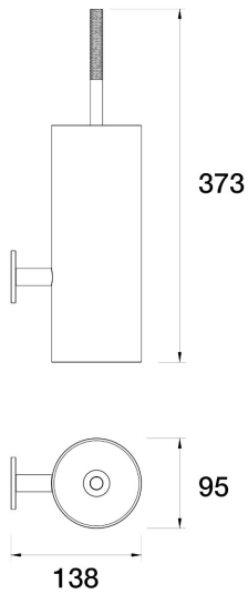
Elm Toilet Brush Holder E40.052.1.44 - Antique Copper
