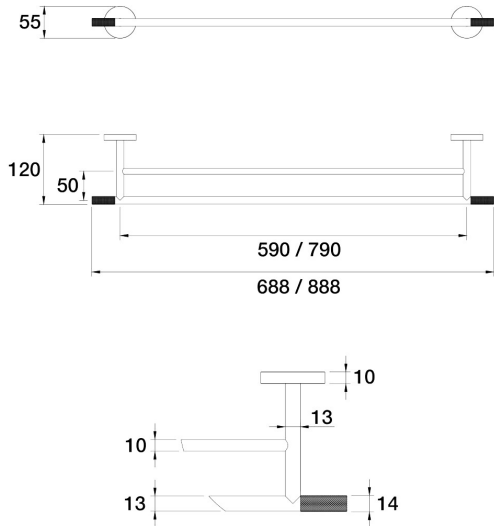
Elm Towel Rail Double 688mm E40.072.1.44 - Antique Copper
