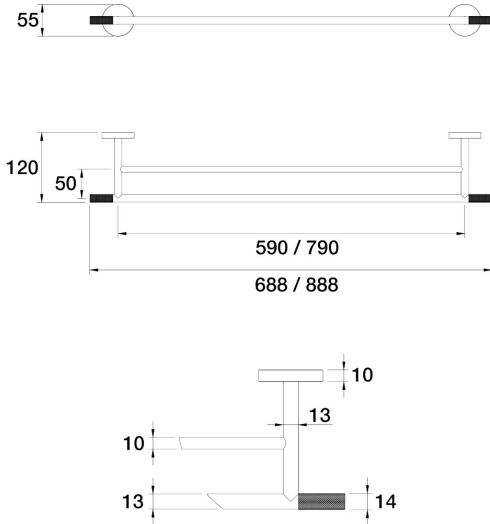
Elm Towel Rail Double 688mm E40.072.1.52 - Burnished
