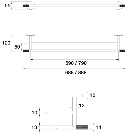
Elm Towel Rail Double 688mm E40.072.1.57 - Matt Nickel
