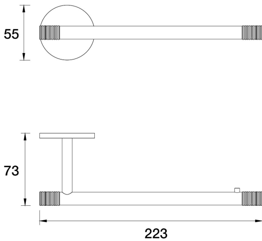
Elm Lane Guest Towel Holder E42.041.1.24 - Brushed Gunmetal
