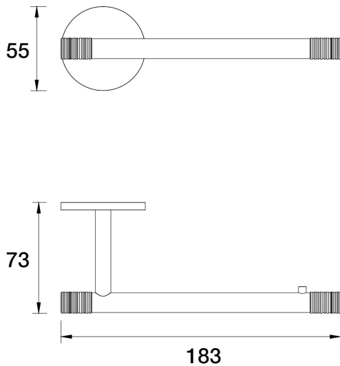
Elm Lane Toilet Roll Holder E42.051.1.27 - Satin Pearl
