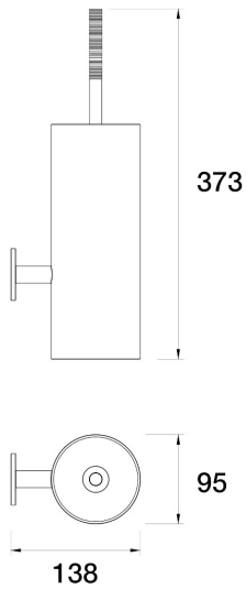
Elm Lane Toilet Brush Holder E42.052.1.32 - Midnight Black
