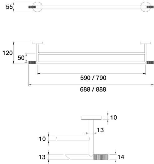
Elm Lane Towel Rail Double 690mm E42.072.1.44 - Antique Copper
