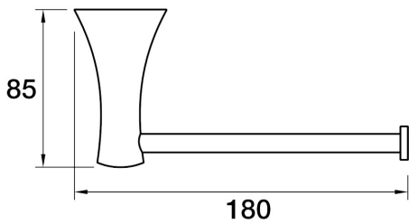
ARI Toilet Roll Holder E43.051.1.45 - Native Brass
