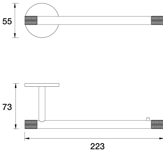
Opus Guest Towel Holder E45.041.1.25 - Brushed Nickel
