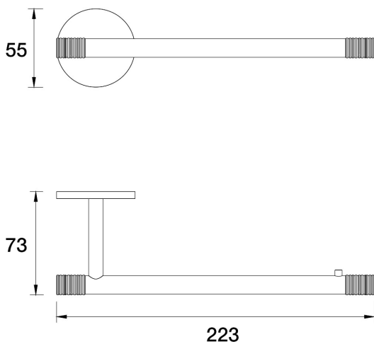
Opus Guest Towel Holder Lane E45.041.2.44 - Antique Copper
