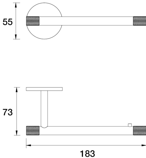
Opus Toilet Roll Holder E45.051.1.27 - Satin Pearl
