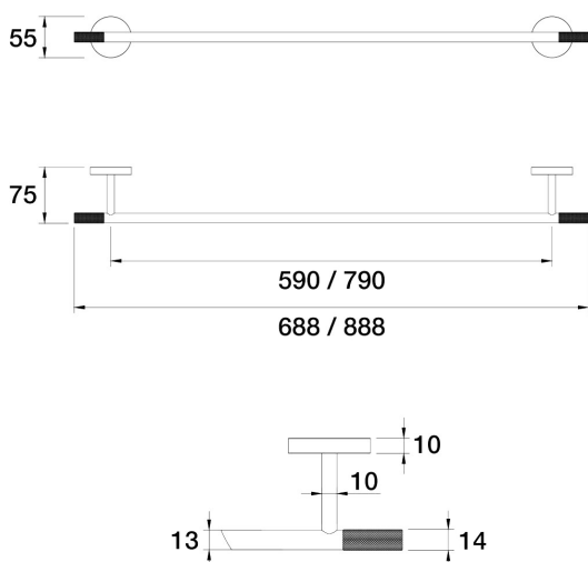
Opus Towel Rail Single 688mm E45.071.1.42 - Brushed Copper
