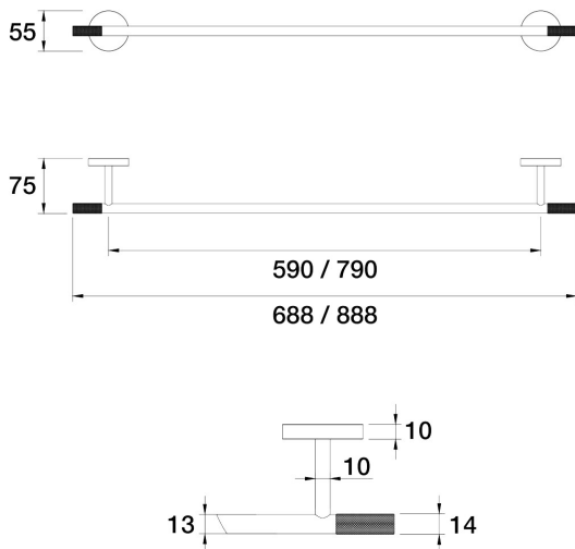
Opus Towel Rail Single 888mm E45.071.2.12 - 23k Brushed Gold
