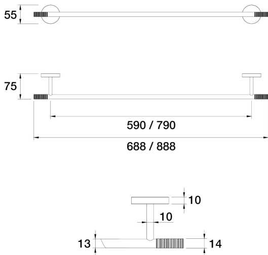
Opus Towel Rail Single Lane 688mm E45.071.3.67 - Vintage Brass
