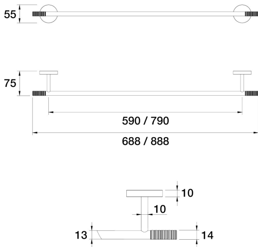
Opus Towel Rail Single Lane 888mm E45.071.4.68 - Autumn Bronze
