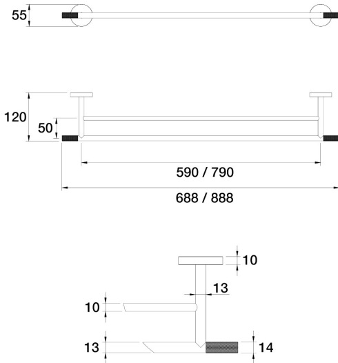
Opus Towel Rail Double 688mm E45.072.1.12 - 23k Brushed Gold
