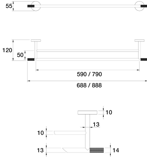
Opus Towel Rail Double 688mm E45.072.1.52 - Burnished
