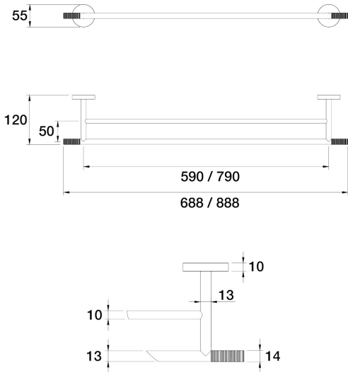
Opus Towel Rail Double Lane 688mm E45.072.3.54 - Volcanic Grey
