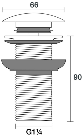
Universal Waste 32mm Mushroom Overflow F11.012.2.01 - Chrome
