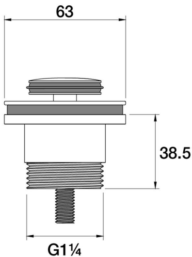
Universal Waste 32mm split Pop Up F11.013.1.01 - Chrome
