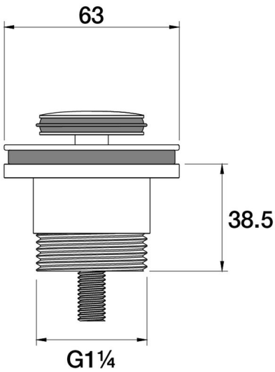
Universal Waste 32mm Split to suit overflow or non overflow Basin F11.013.1.01 - Chrome
