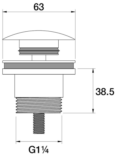
Universal Waste 32mm split Mushroom Pop Up F11.013.2.39 - Antique Bronze
