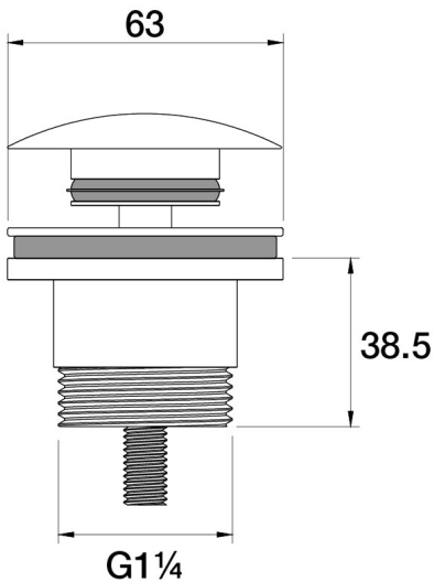
Universal Waste 32mm split Mushroom Pop Up F11.013.2.41 - Brushed Brass
