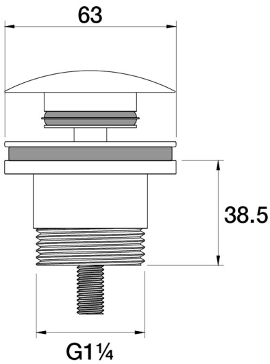
Universal Waste 32mm split Mushroom Pop Up F11.013.2.54 - Volcanic Grey
