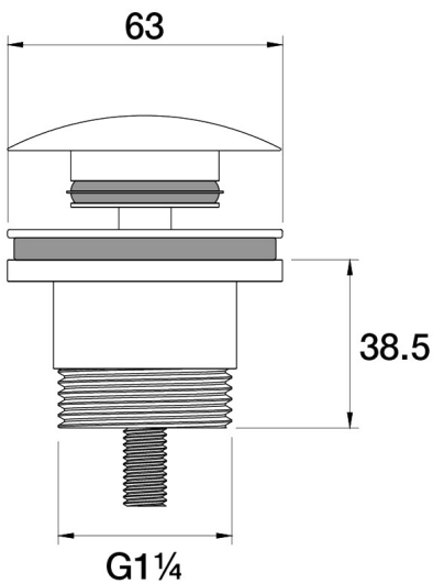
Universal Waste 32mm split Mushroom Pop Up F11.013.2.57 - Matt Nickel
