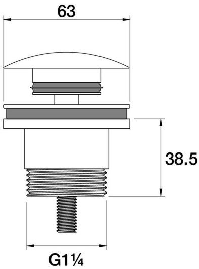
Universal Waste 32mm split Ceramic Mushroom Tap P013.3.01 - Chrome
