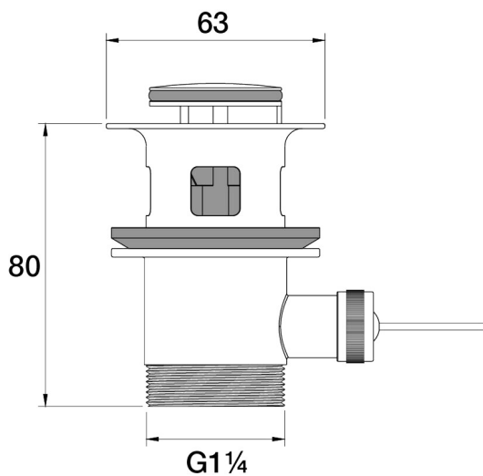
Universal Waste 32mm Bidet Overflow F11.014.2.12 - 23k Brushed Gold
