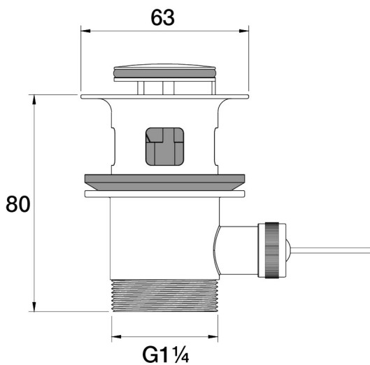
Universal Waste 32mm Bidet Overflow F11.014.2.24 - Brushed Gunmetal
