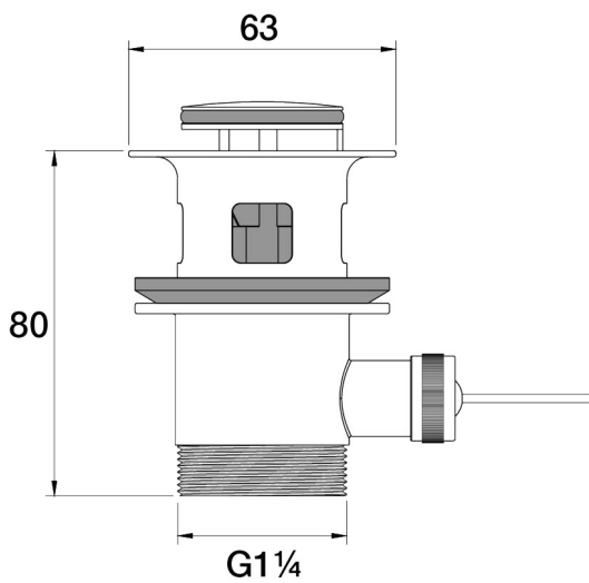
Universal Waste 32mm Bidet Overflow F11.014.2.48 - Copper
