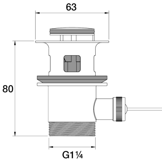
Universal Waste 32mm Bidet Overflow F11.014.2.57 - Matt Nickel
