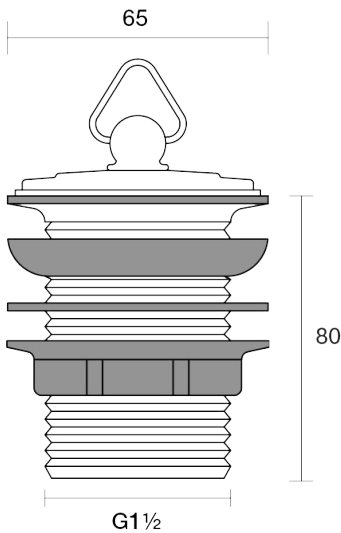
Universal Waste 40mm Standard F11.021.1.01 - Chrome
