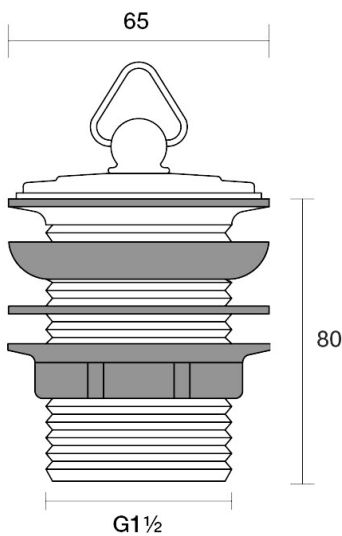
Universal Waste 40mm Standard F11.021.1.11 - 23k Gold
