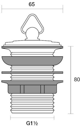
Universal Waste 40mm Standard F11.021.1.39 - Antique Bronze
