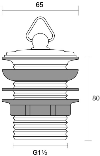
Universal Waste 40mm Standard Overflow F11.021.2.12 - 23k Brushed Gold
