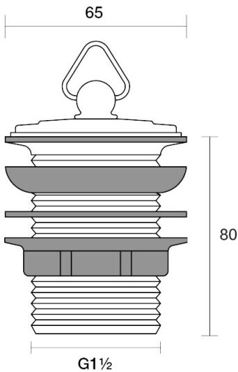
Universal Waste 40mm Standard Overflow F11.021.2.24 - Brushed Gunmetal
