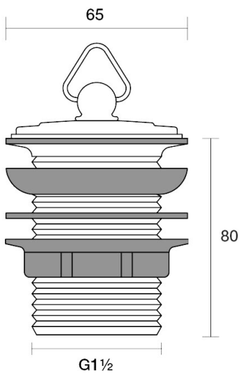
Universal Waste 40mm Standard Overflow F11.021.2.54 - Volcanic Grey
