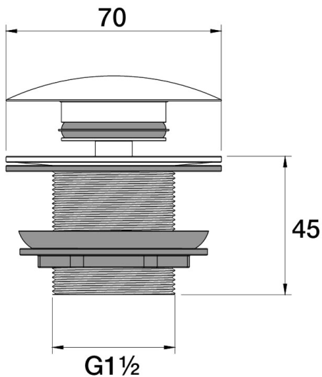
Universal Waste 40mm To Suit Bath F11.022.1.21 - Brushed Rose Gold
