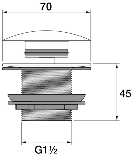
Universal Waste 40mm To Suit Bath F11.022.1.43 - Brass
