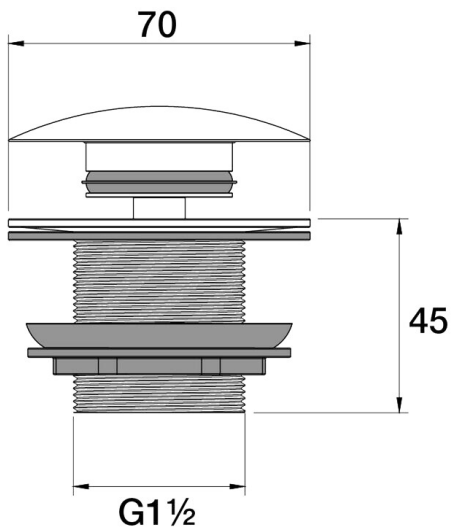
Universal Waste 40mm To Suit Bath F11.022.1.44 - Antique Copper
