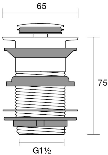
Universal Waste 40mm Pop - Up F11.023.1.11 - 23k Gold
